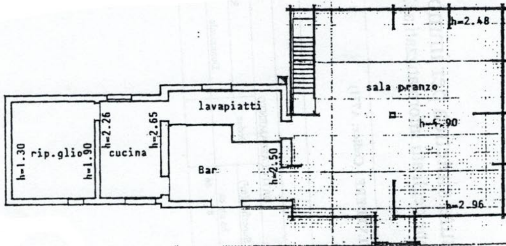
PIANO TERRA
