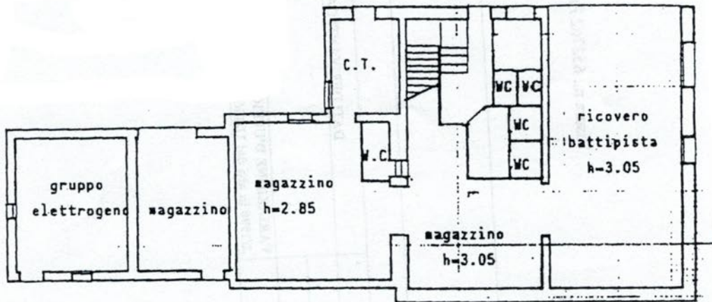
PIANO SEMINTERRATO
